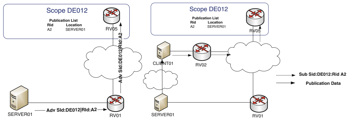
Fig. 1 a Publication (advertisement) and b subscription procedures in the PSI architecture
