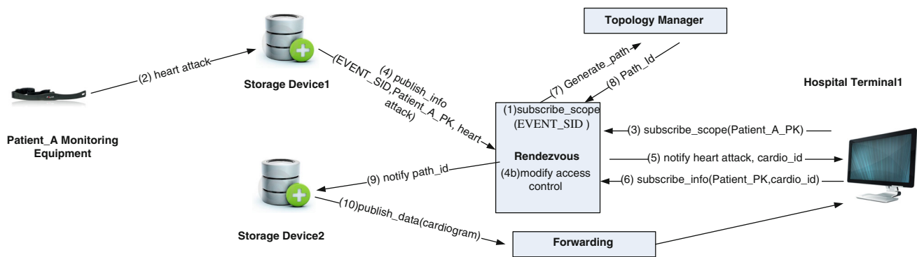
Fig. 4 Messages exchanged in case of emergency
