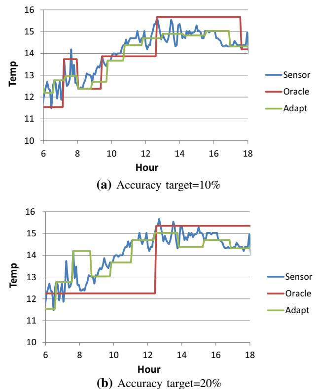
Fig. 3 Measurements with the Oracle and the AIMD adaptation procedure for two target accuracies: 10% and 20%. Comparison of the two graphs illustrates the trade-off between the target data accuracy and the number of measurements
