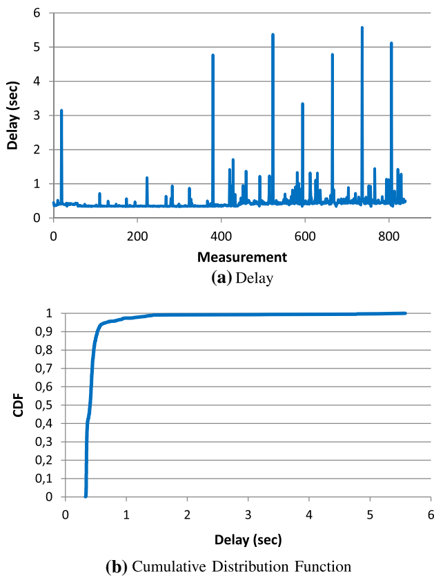
Fig. 5 Delay to receive response from the FIESTA-IoT platform. Although the average FIESTA-IoT response time is small, approximately equal to 0.47 s, the response time can result in values which are above 5 s
