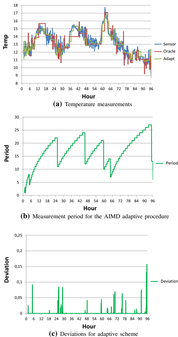
Fig. 4 Performance of the AIMD adaptation procedure in a 96 h time window of temperature measurements from SmartSantander, where sensors provide measurements every 5 min. Accuracy target = 10%
