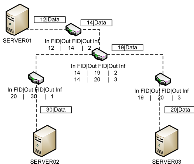
Fig. 8 PSIRP forwarding
