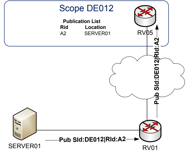
Figure 1: Publication in the \Psi architecture
