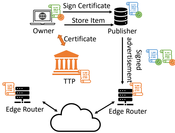
Fig. 1. Trust relationships in legacy NDN routing. Edge routers are configured with the certificate of the TTP. The TTP issues a certificate to the owner and the owner issues a certificate to the publisher. The publisher includes both certificates in the advertisement.
