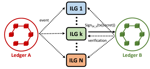
Fig. 4. Decentralized interledger gateway architecture where the ILGs are operated by different organizations. One of the N ILGs (ILG k in the figure) is selected to submit the transaction to ledger B. The selection is based on the hash of the last or the next block mined on ledger B. ILGs use different accounts to submit transactions to ledger B.
