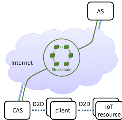
Fig. 2. Both the client and the IoT resource have only D2D connectivity. Prior to requesting access, the client must obtain the authorization credentials from the CAS. Once it has the credentials, the client can request access to the resource using D2D communication, without requiring synchronous network connectivity or simultaneous D2D connectivity with the CAS.
