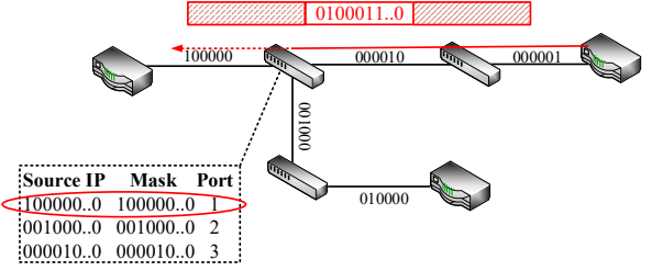
Figure 1: Example of Bloom filter-based forwarding.
