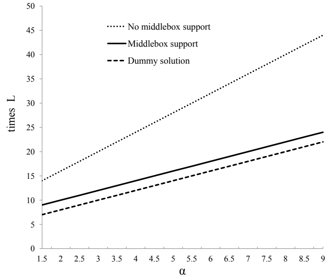
Fig. 3. Time required for the first packet of the publication to reach the subscriber (measured in multiples of the latency L ) as a function of \alpha .
