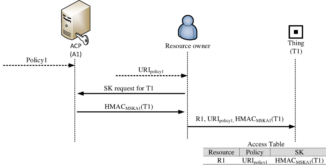
Figure 1. System setup
