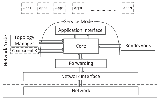
Fig. 2. The Blackadder platform as ICN core node basis
