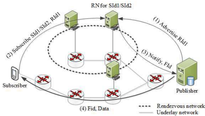
Fig. 1. The Publish-Subscribe Internet architecture
