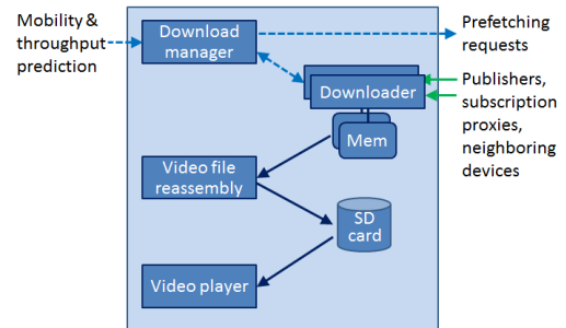
Fig. 3. Multi-source mobile video streaming client design
