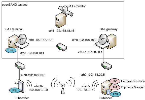
Fig. 2. Testbed overview
