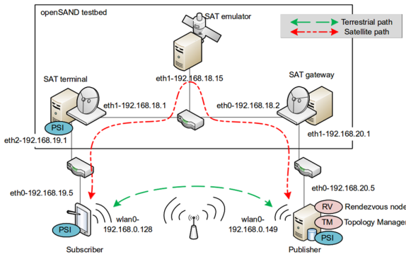
Fig. 5. Setup for the multipath based solution
