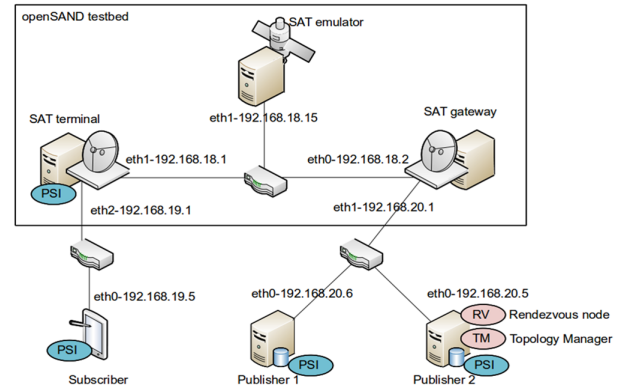
Fig. 6. Setup for the multisource based solution
