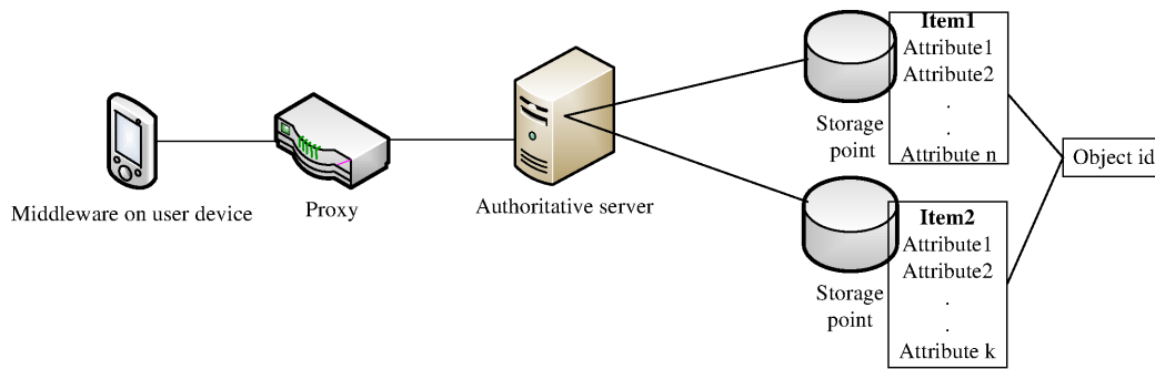
Fig. 1. Architecture components
