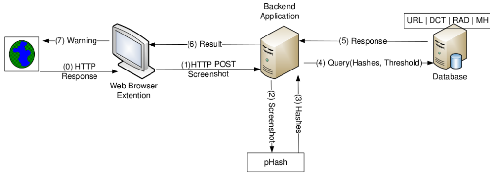
Fig. 2. Implementation overview
